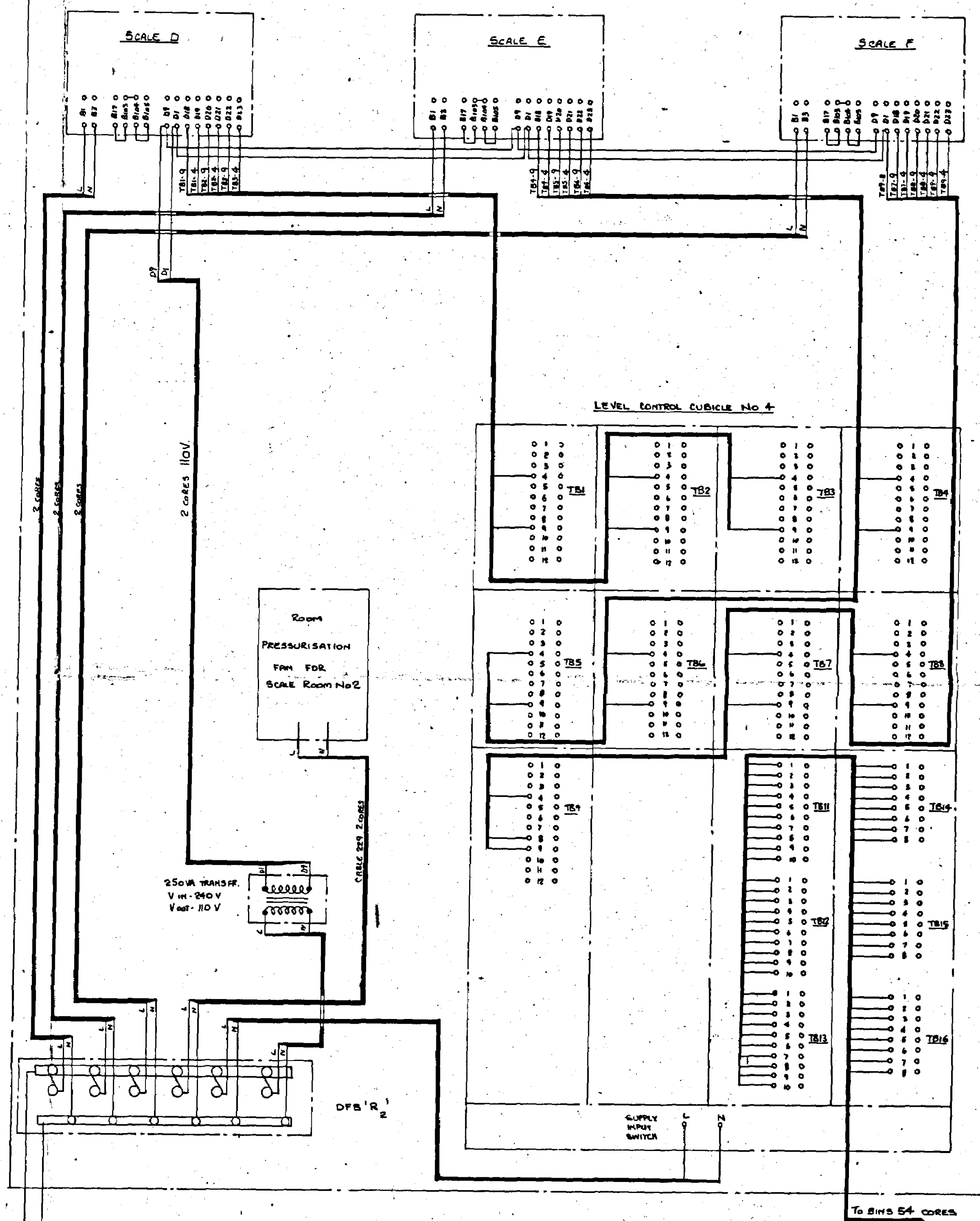
INTERCONNECTION DIAGRAM FOR LORRY LOADING SCALE ROOMS Nos 1 & 2
